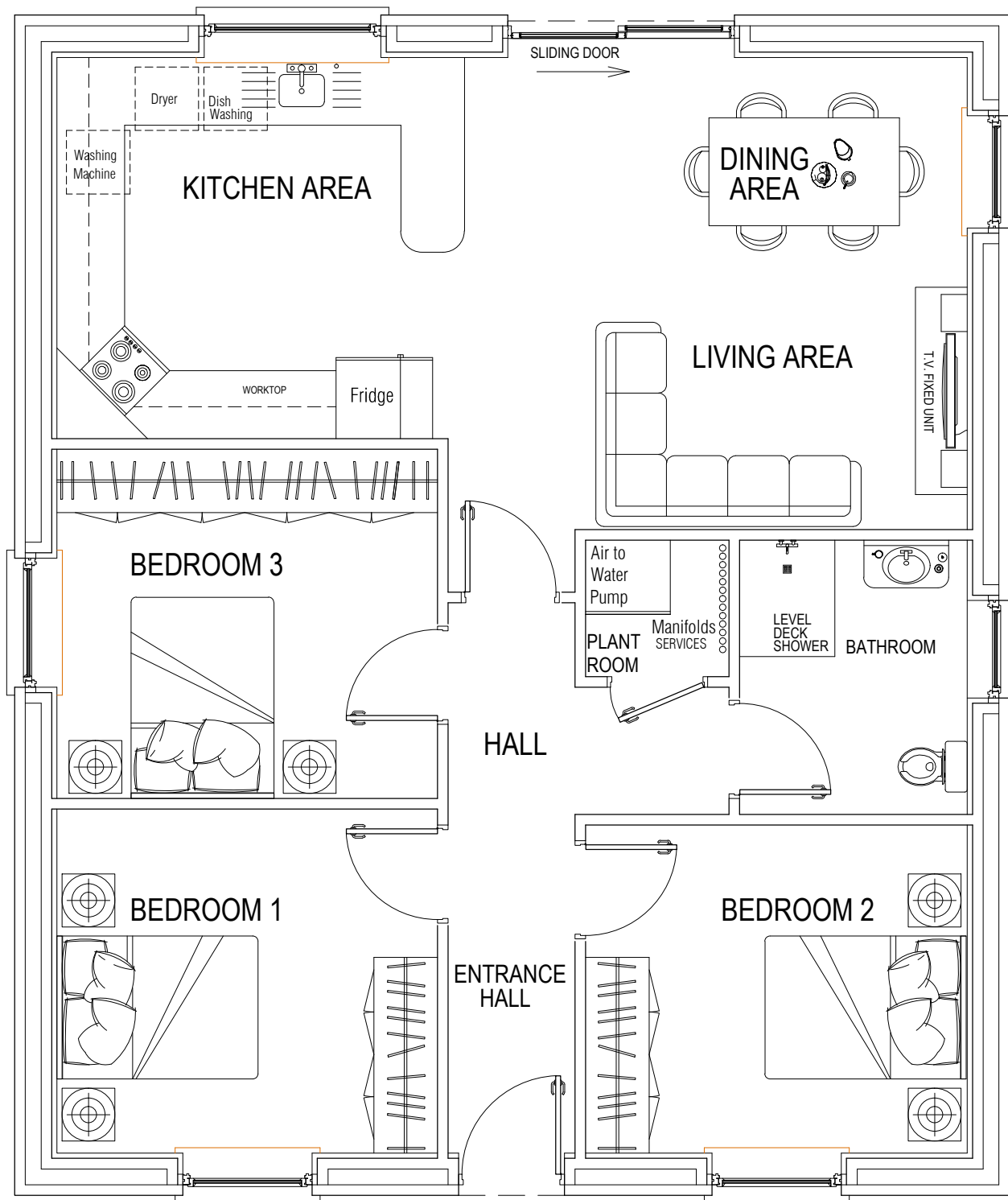
FLOOR PLAN
